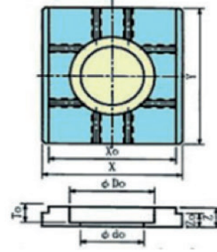
Lower Movable Die Changing Bolster
