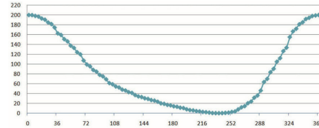
YM-600 Stroke Motion Curve
